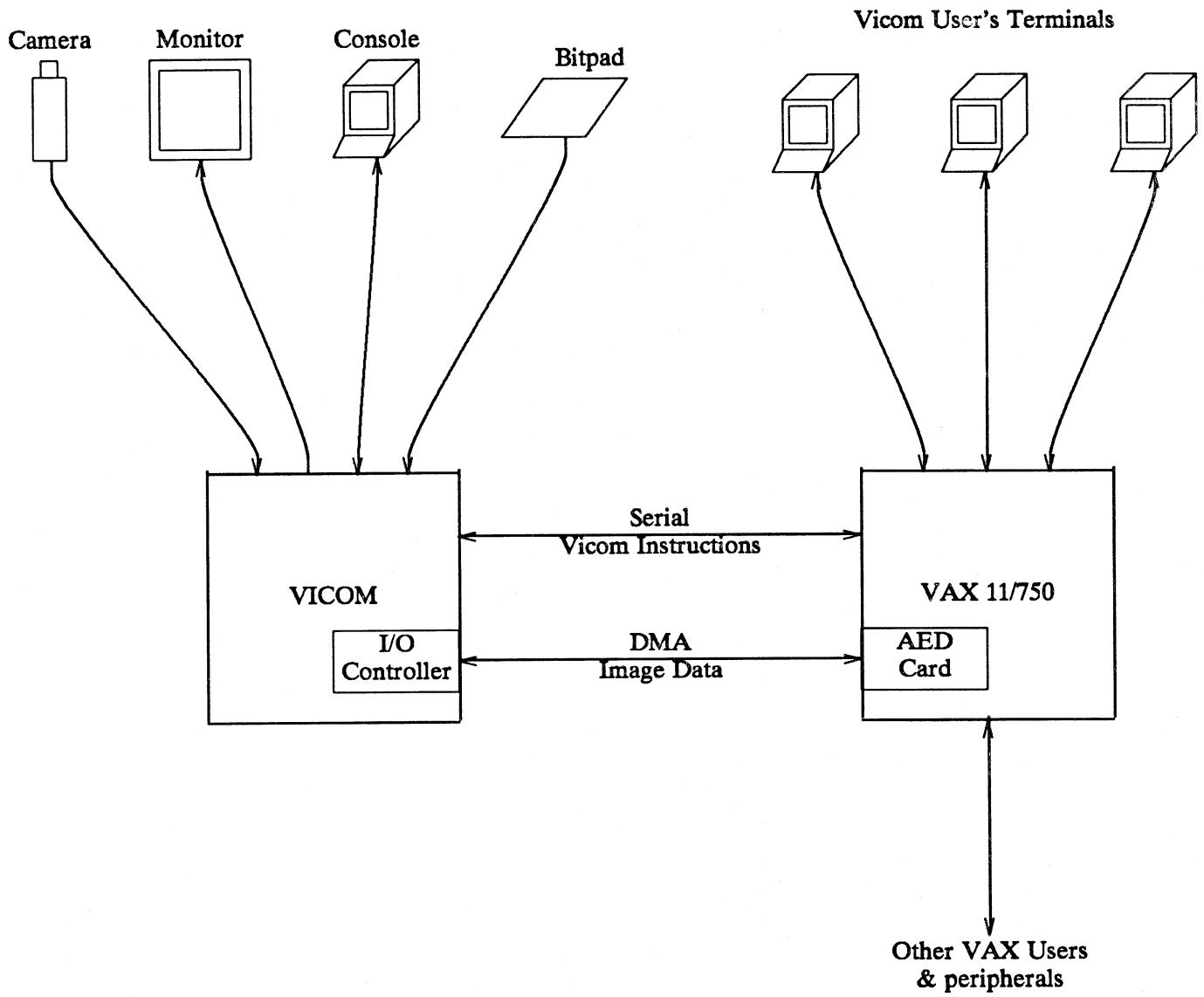
Figure 2.1. VICOM/host configuration.
